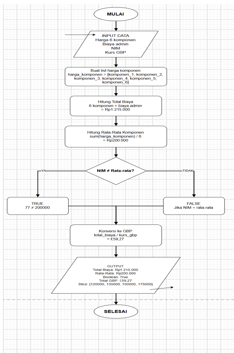
Gambar 1.1 Flowchat draw.io
